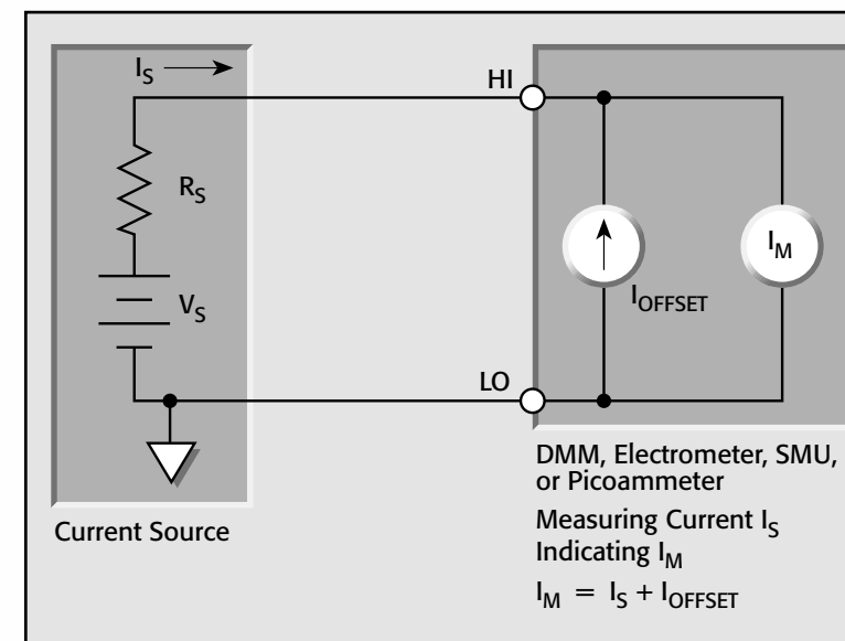
Figure 6: Effects of Input Offset Current on Current Measurement Accuracy
